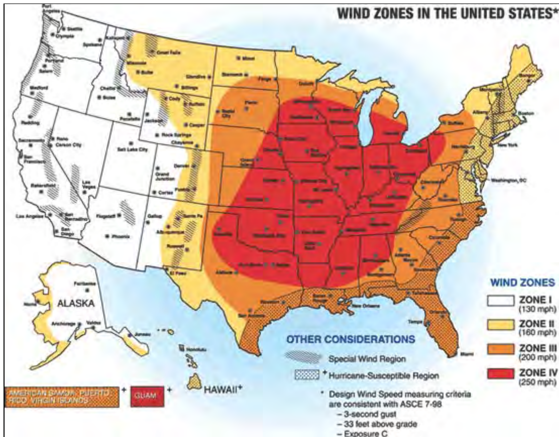
Figure 4.3 Wind Zones in the United States
