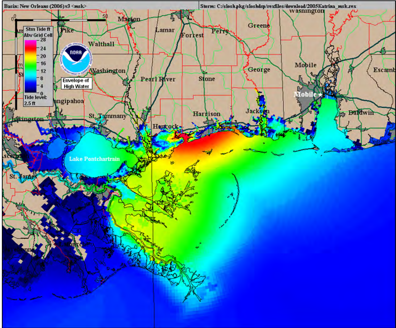
Map 4.3 SLOSH Model Hurricane Katrina (Source NHC)
